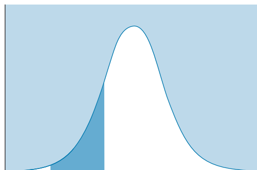
FIGURE 7.3.3 The probability of falling within a region that is farther from the middle of the curve. Since the normal curve is lower here, the probability is smaller than that shown in Figure 7.3.2.
