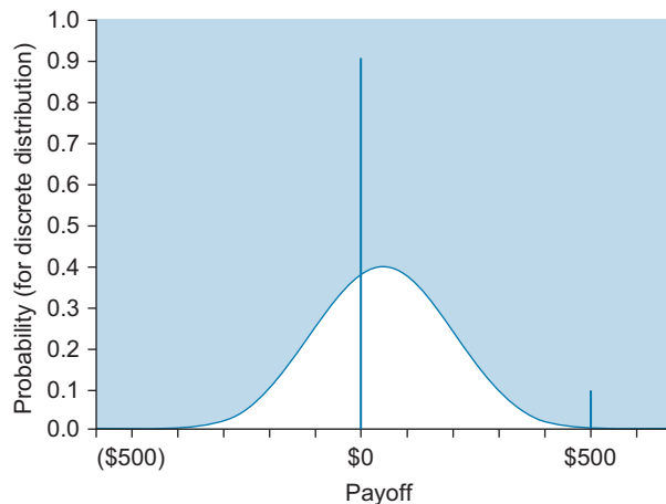
FIGURE 7.3.11 The discrete distribution of the payoff and the normal distribution having the same mean ($50) and standard deviation ($150). These distributions and their probabilities are very different. The discrete distribution gives the correct answers; the assumption of normality is wrong in this case.
