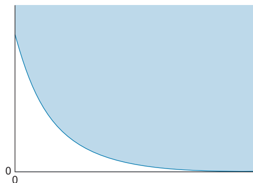
FIGURE 7.5.4 The exponential distribution is a very skewed distribution that is often used to represent waiting times between events.
