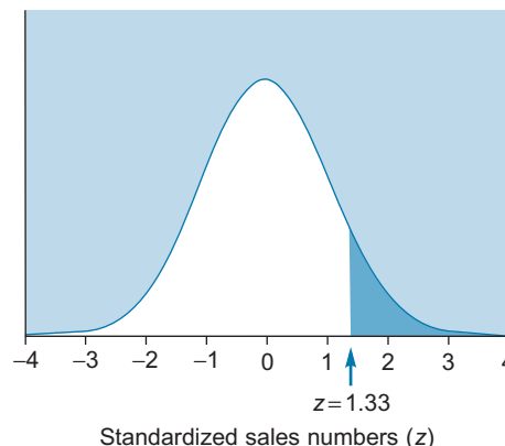
FIGURE 7.3.8 The probability of a really good quarter, in terms of standardized sales numbers. The shaded area is 1 minus the unshaded area under the curve, which may be looked up in the table. The answer is 0.0918.
