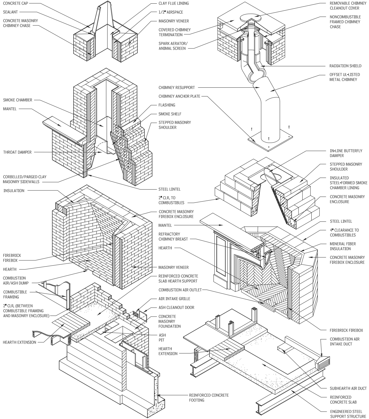
TRADITIONAL CONSTRUCTION TECHNIQUE
